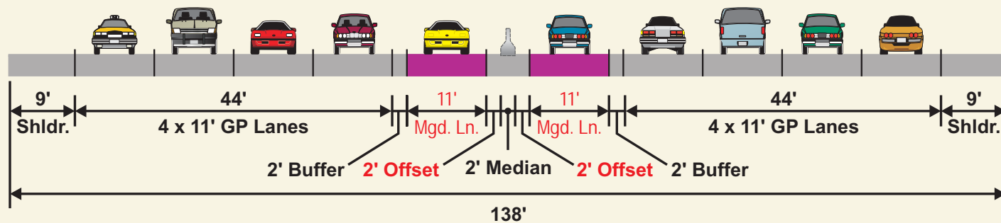
RESTRIPIING - 11' Lanes With Reduced Right Shoulder and Managed Lanes Buffer
