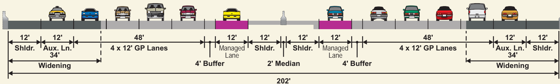
ALTERNATIVE 1
