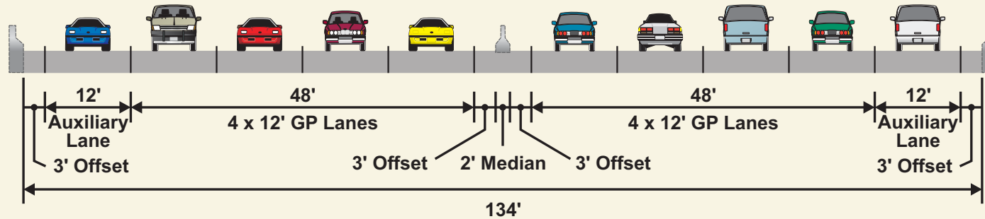
EXISTING CONDITIONS
