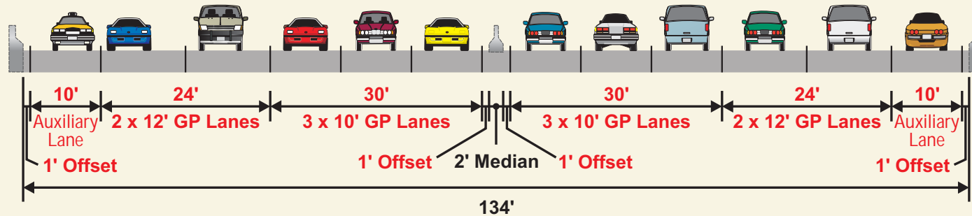
RESTRIPING OPTION A
