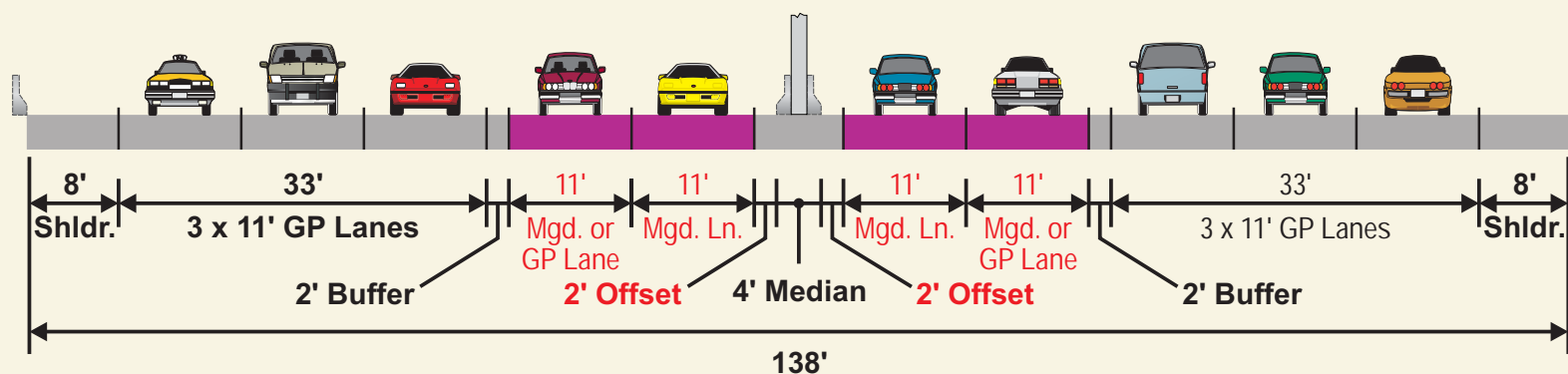
Reduced Typical Section at Median Bridge Piers
