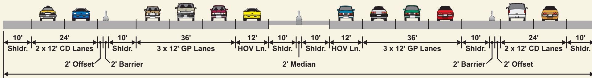
214' EXISTING CONDITIONS
