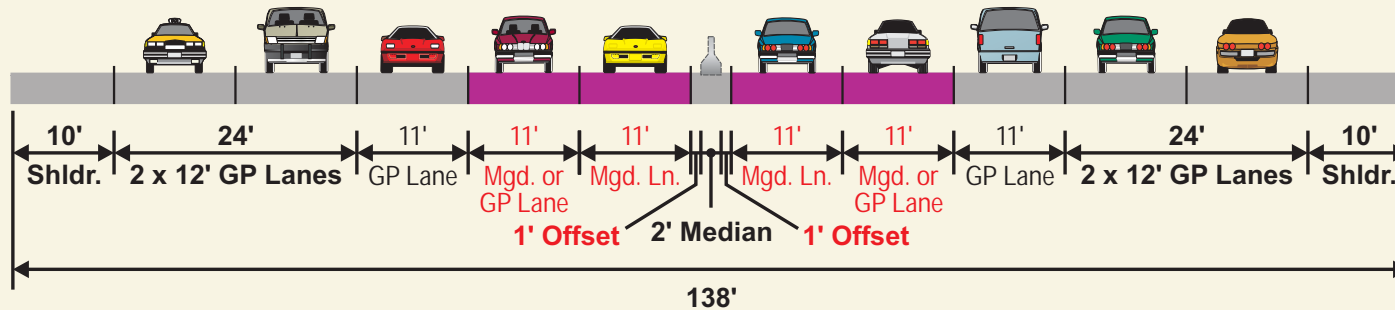
LEFT SHOULDER USE
