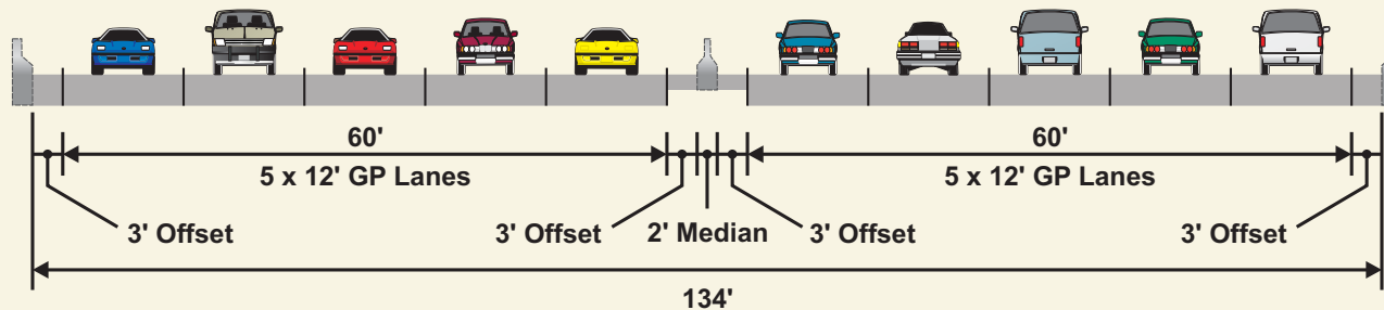
EXISTING CONDITIONS
