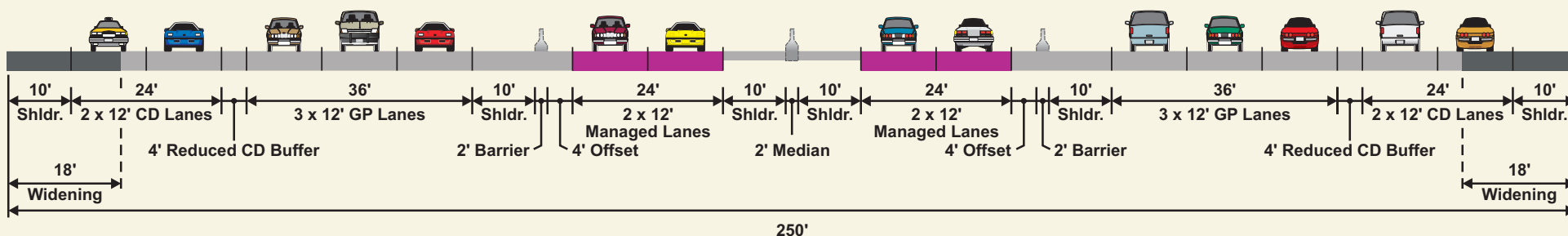
ALTERNATIVE 4
