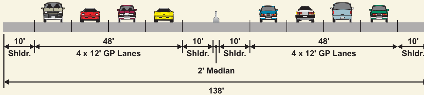
EXISTING CONDITIONS
