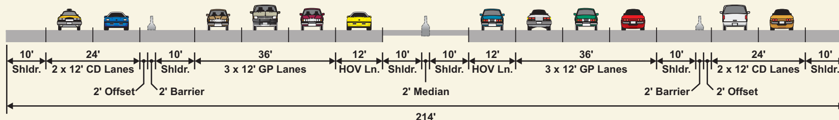
EXISTING CONDITIONS
