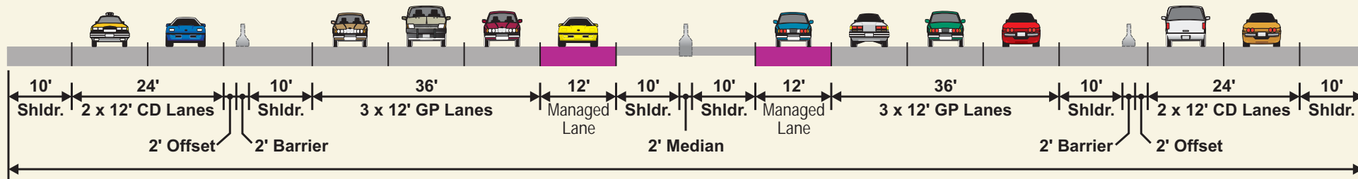
214' ALTERNATIVE 1
