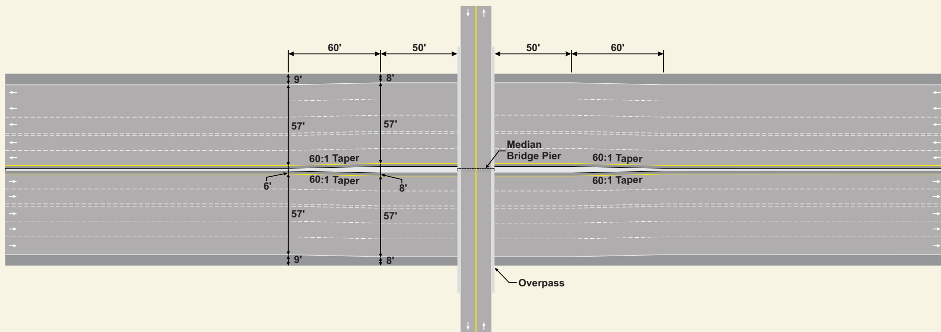
Lane Transition at Median Bridge Pier
